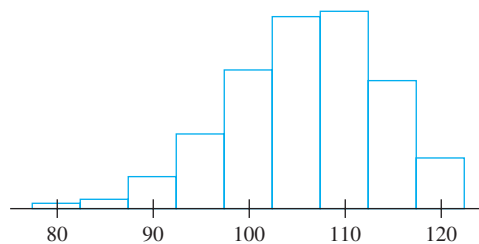
Figure 5.9 Probability histogram for \bar{X} based on n = 4 in Example 5.21
