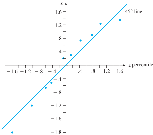
Figure 4.33 Plot of pairs ( z percentile, observed value) for the data of Example 4.29
