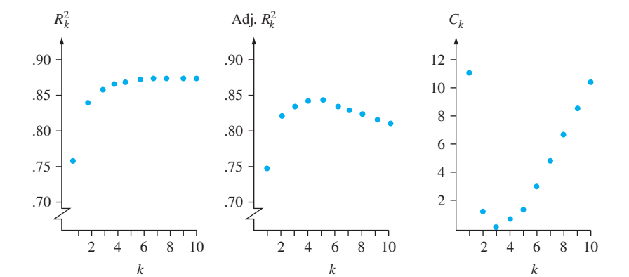
Figure 13.21 R_k^2 and C_k plots for the gas mileage data
