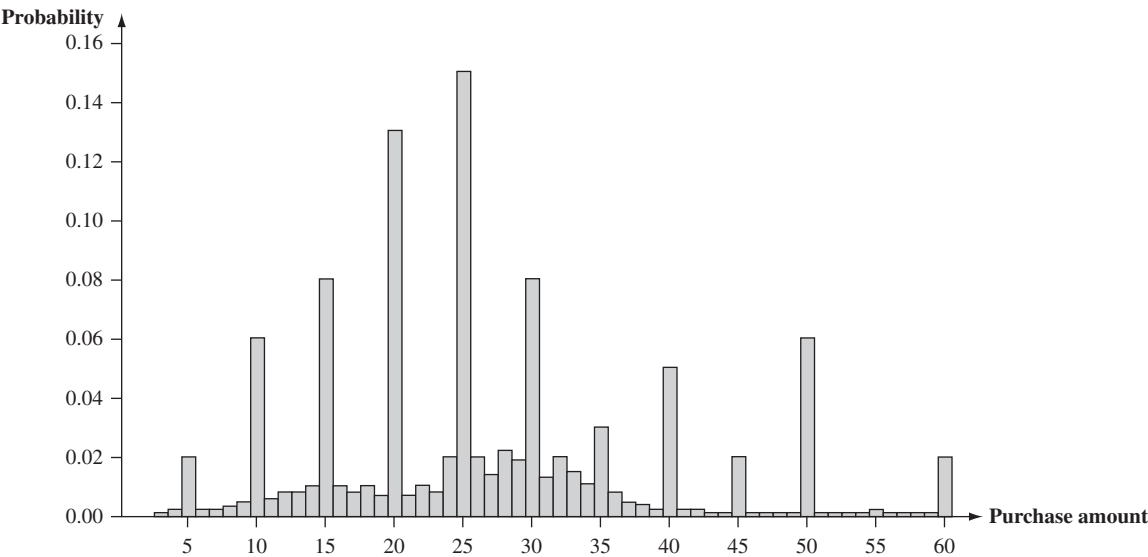
Figure 5.17 Probability distribution of X = amount of gasoline purchased ($)
