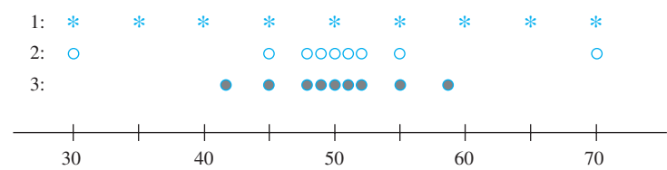
Figure 1.18 Samples with identical measures of center but different amounts of variability
