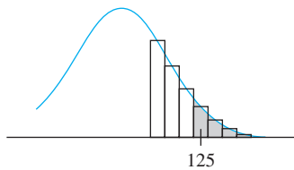
Figure 4.24 A normal approximation to a discrete distribution
