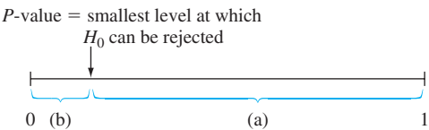
Figure 8.1 Comparing \alpha and the P -value: (a) reject H_0 when \alpha lies here; (b) do not reject H_0 when \alpha lies here
